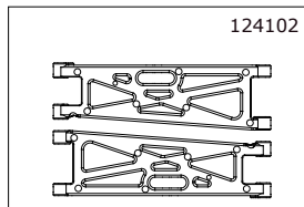
Unterer Querlenkersatz vorne - S10 Twister SC Front Lower Suspension Arm Set - S10 Twister SC
