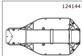
Chassisplatte - S10 Twister SC Chassis Plate - S10 Twister SC
